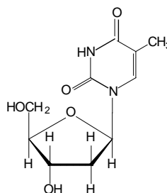
Timidin dT
