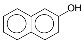
\beta -naftol
