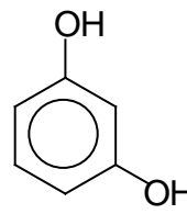
m -izomer
